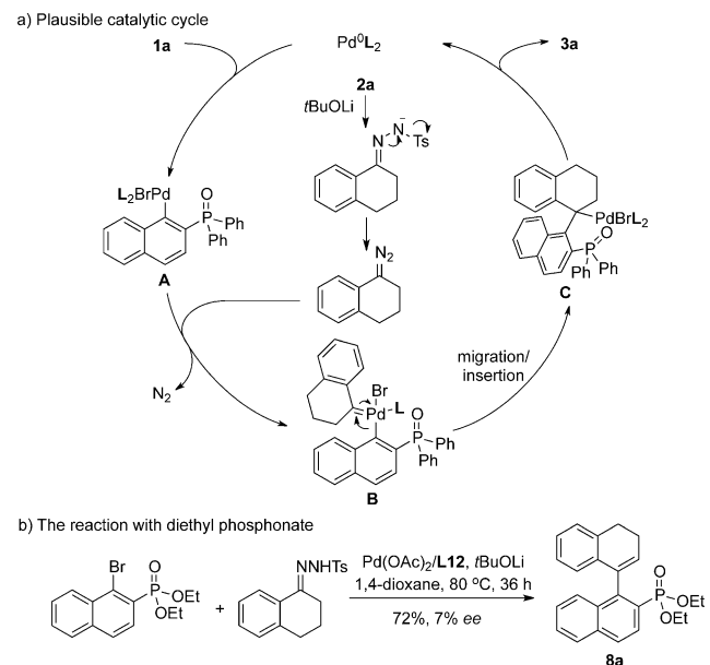
Scheme 4. Plausible catalytic cycle.
